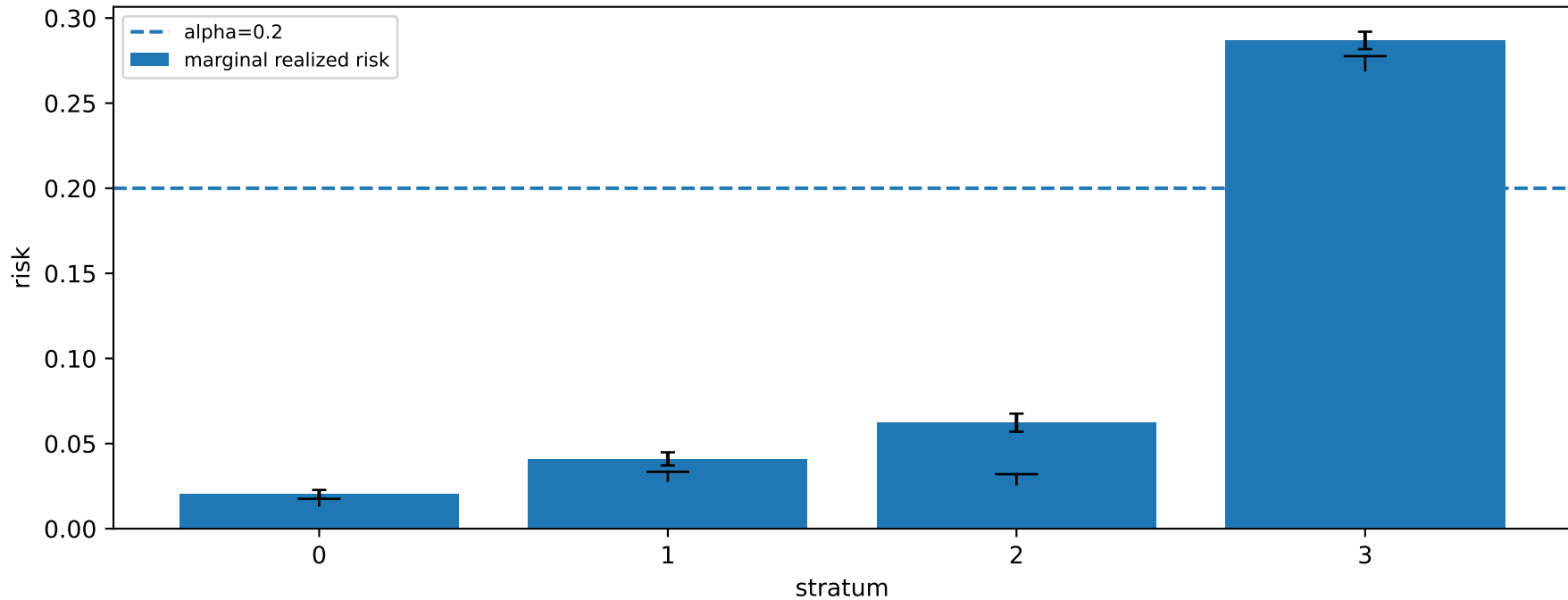
F2 per-stratum marginal risk -- tabular-adult[margin] ts0 greedy lambda_ref=0.9
